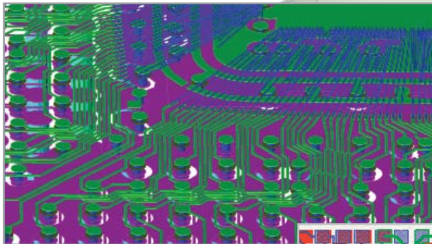
ADS Layout information is combined with the Momentum substrate definition to produce a 3D spatial representation of circuit geometries.
