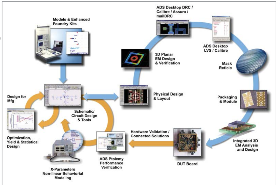
The Complete MMIC ADS Desktop Design Flow enable front-to-back design and simulation to physical design, verification and manufacturing.
