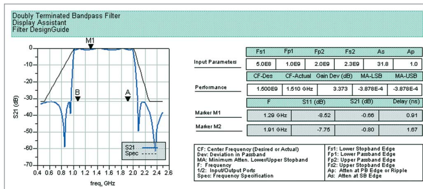
DesignGuides and templates in ADS make displaying simulation results easy.
